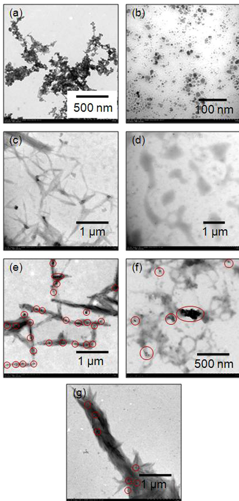
Fig. 3. TEM micrographs of (a) MAG, (b) O-MAG, (c) CTWK, (d) WSCS, (e) CTWK-MAG, (f) WSCS-MAG, and (g) CTWK-MAG under magnetic field. Circles in figure (e–g) indicate MAG.
