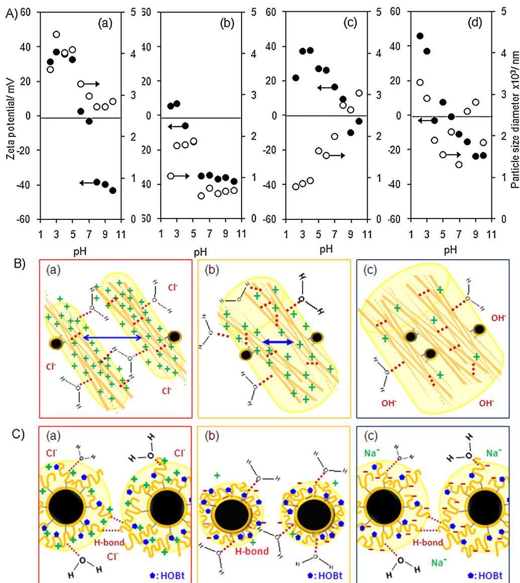
Fig. 6. (A) Zeta potential and particle size of (a) MAG, (b) S-MAG, (c) CTWK-MAG, and (d) WSCS-MAG at pH 2.2–10 in water (pH adjusting by NaOH and HCl); (B) schematic illustrations of CTWK-MAG in water at (a) pH 2–4, (b) pH 5–7, and (c) pH 8–10; and (C) schematic illustrations of WSCS-MAG in water at (a) pH 2–3, (b) pH 3–7, and (c) pH 8–10.
