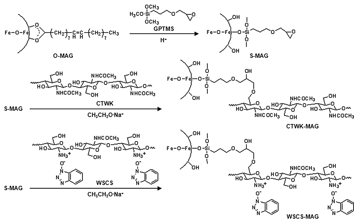
Scheme 1. Preparation of CTWK-MAG and WSCS-MAG.
