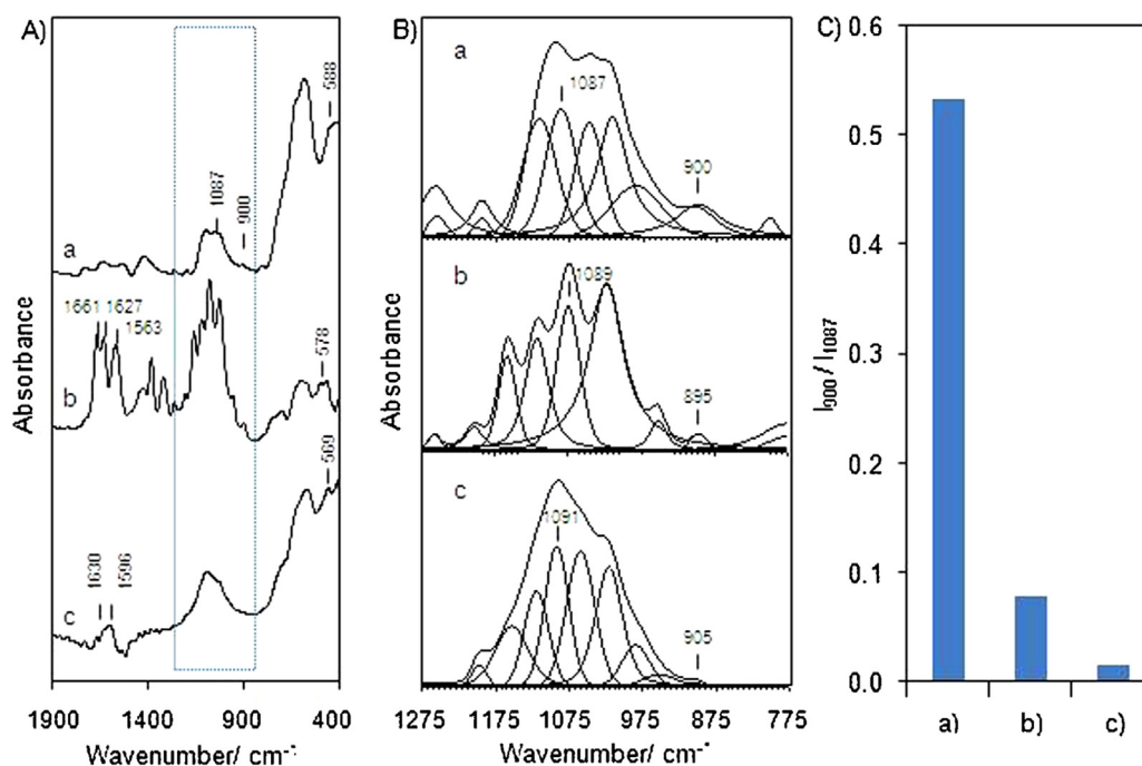
Fig. 1. (A) FTIR spectra of (a) S-MAG, (b) CTWK-MAG, and (c) WSCS-MAG; (B) curve fitting of (a) S-MAG, (b) CTWK-MAG, and (c) WSCS-MAG; and (C) integral ratio of oxirane peak at 900 cm -1 to Si-O peak at 1087 cm -1 of (a) S-MAG, (b) CTWK-MAG, and (c) WSCS-MAG.
