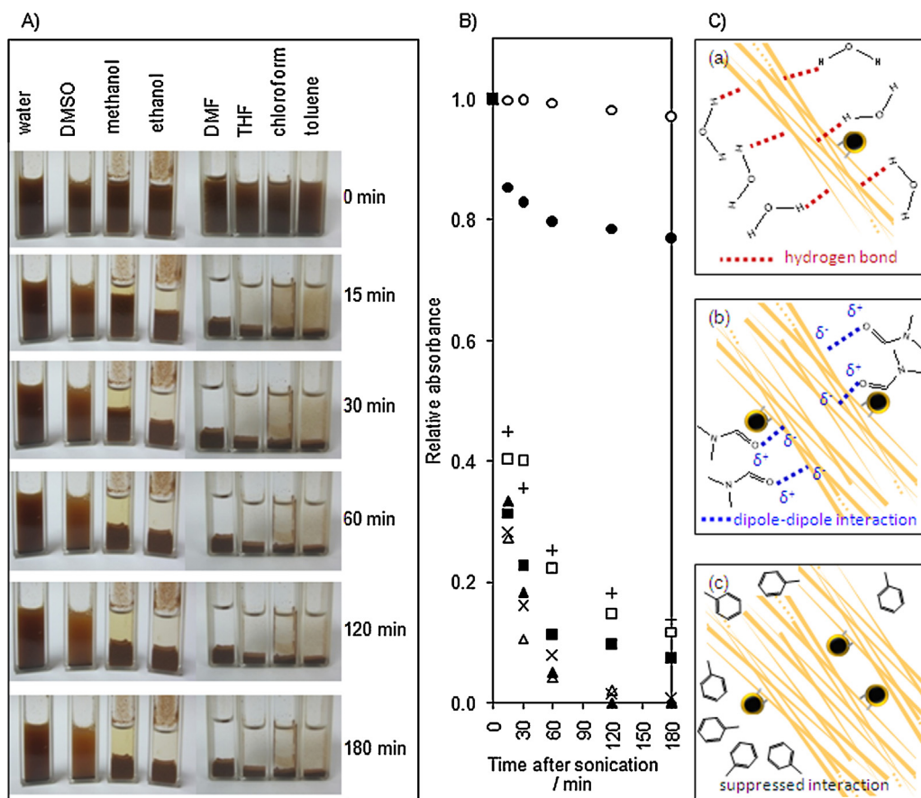
Fig. 5. (A) Photographs of CTWK-MAG dispersed in various solvents in relation to the dielectric constant value ( k ): toluene ( k=2.38 ), chloroform ( k=4.81 ), THF ( k=7.58 ), DMF ( k=19.9 ), ethanol ( k=24.5 ), methanol ( k=32.7 ), DMSO ( k=46.7 ), and water ( k=80.1 ) at 0 min, 30 min, 60 min, 120 min, and 180 min after sonication; (B) relative absorbance of CTWK-MAG in various solvents: water (○), DMSO (●), methanol (□), ethanol (■), DMF (△), THF (▲), chloroform (+), and toluene (×); and (C) schematic illustration of solvent interactions to CTWK-MAG in (a) water, (b) DMF, and (c) toluene.
